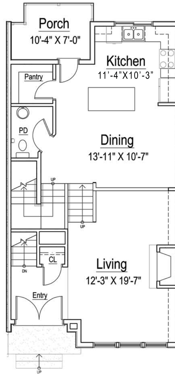
FIRST FLOOR
